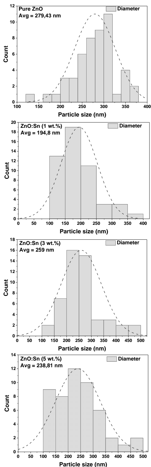
Fig. 7. SEM images and particle size distribution of pure ZnO and Sn-doped ZnO thin films at different doping concentrations, obtained from SEM analysis
