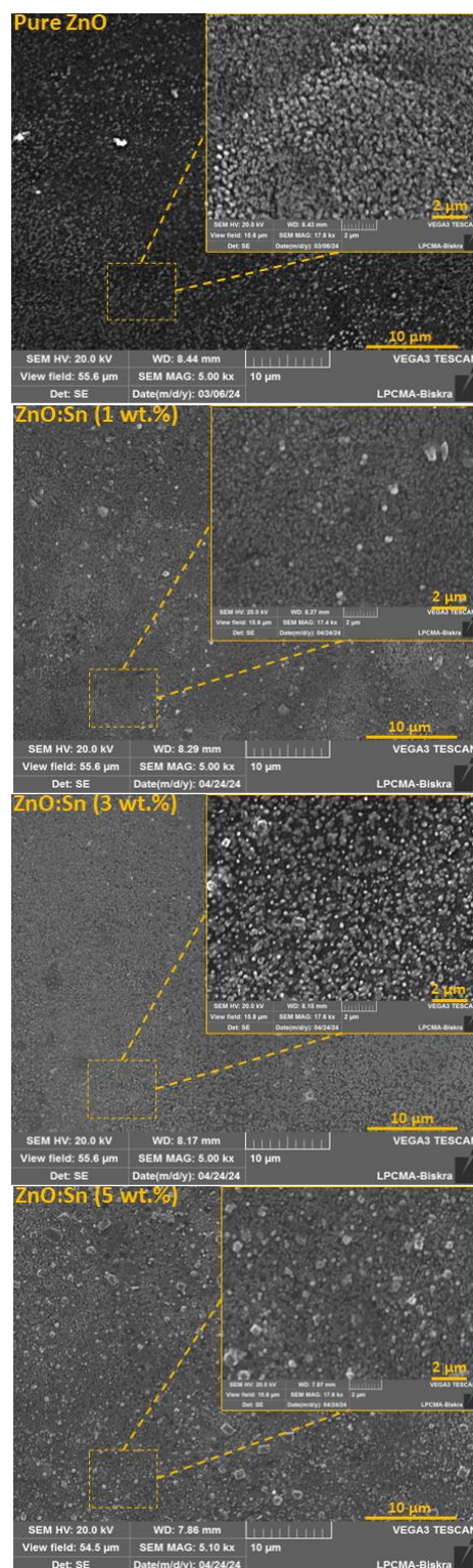
Fig. 7. SEM images and particle size distribution of pure ZnO and Sn-doped ZnO thin films at different doping concentrations, obtained from SEM analysis
